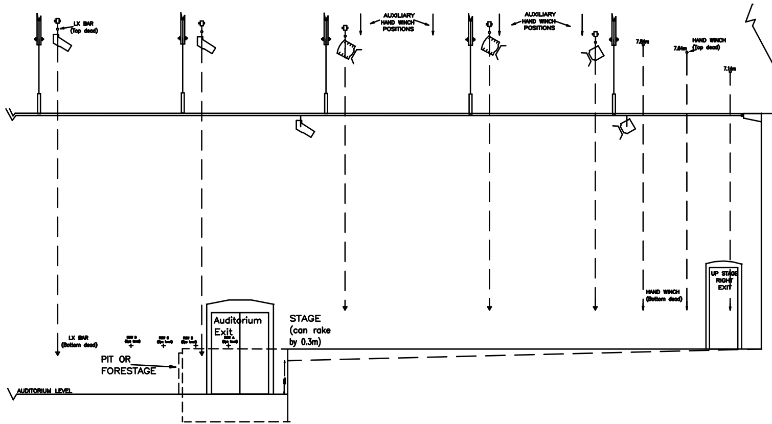
Snape Maltings Concert Hall Elevation Looking S.R. From C.S.
